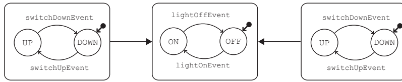
Figure 41: FSM showing a situation where the issue of priority arises
