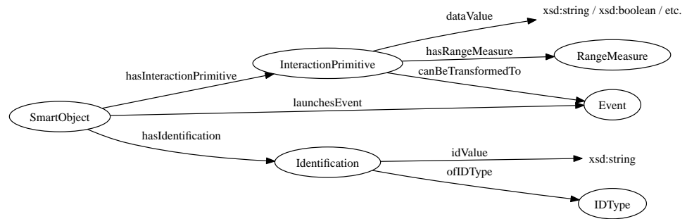
Figure 14: Semantic Interaction Ontology
