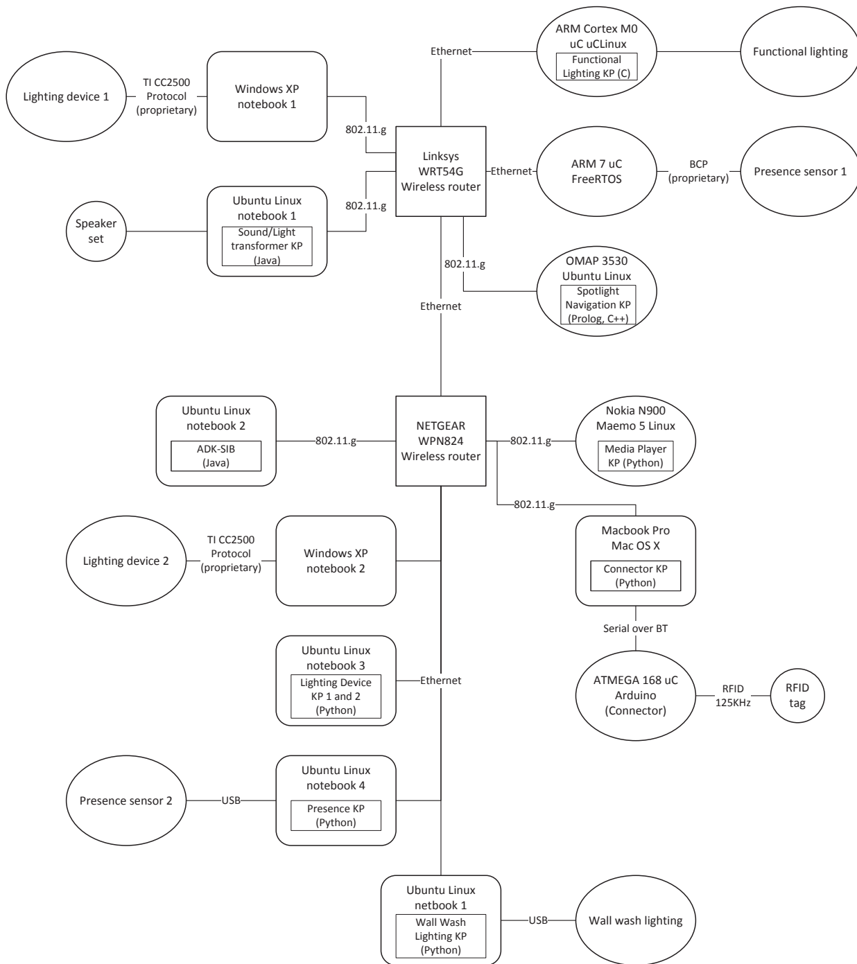
Figure 21: Technical details of the Smart Home pilot
