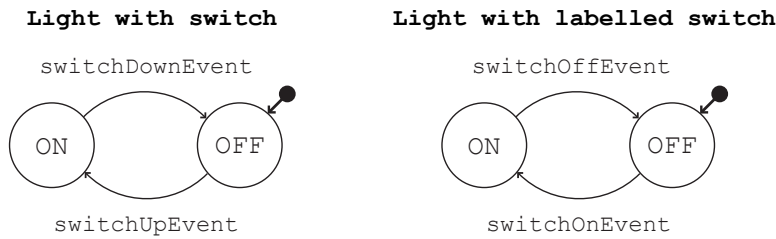
Figure 34: FSMs for a simple light with a switch and a light with a labelled switch
