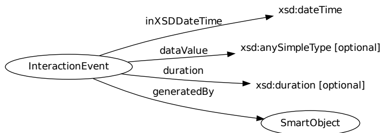
Figure 48: An interaction event as modelled in the ontology
