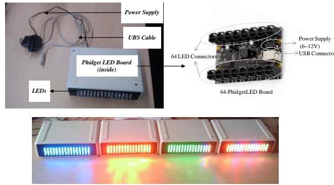
Figure 15: Wall-wash lighting developed by TU/e SAN
