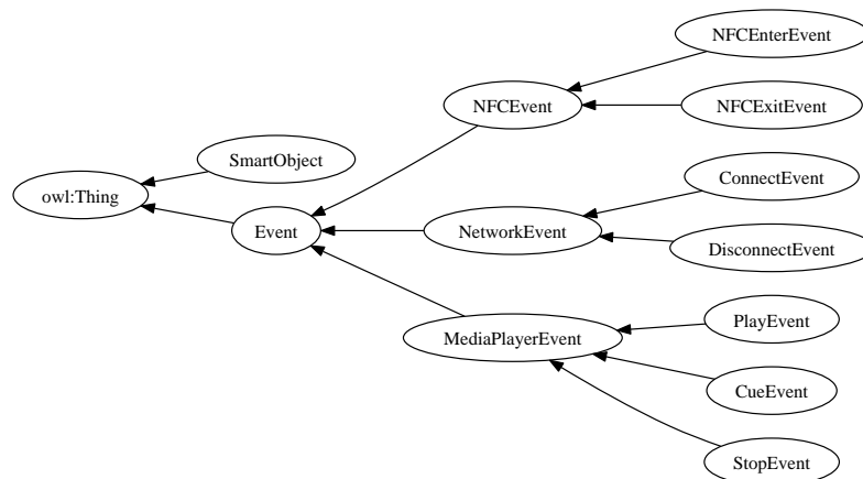
Figure 5: Ontology indicating subclass relationships
