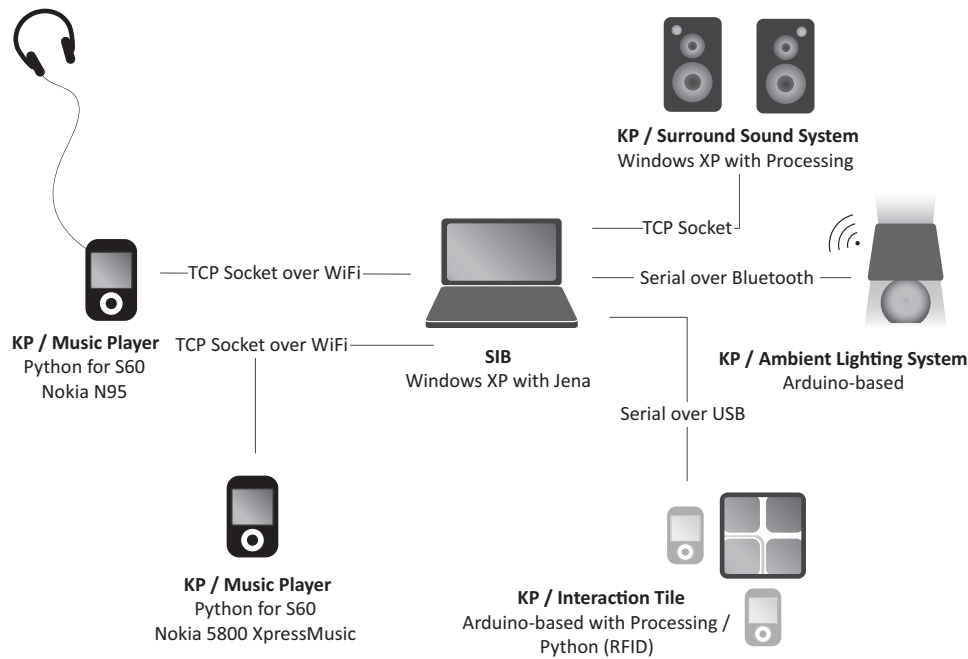
Figure 11: An overview of the demonstrator
