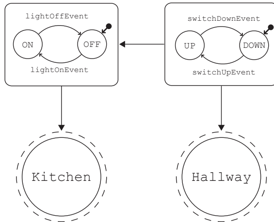
Figure 40: Semantic connections between smart objects and places
