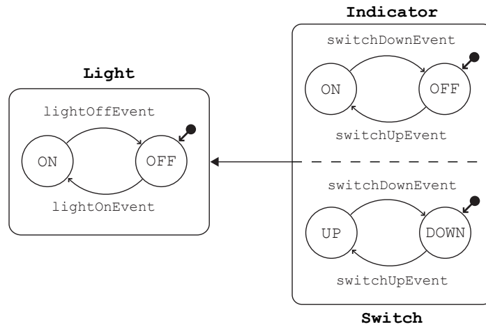
Figure 36: Light connected to light switch with augmented feedback
