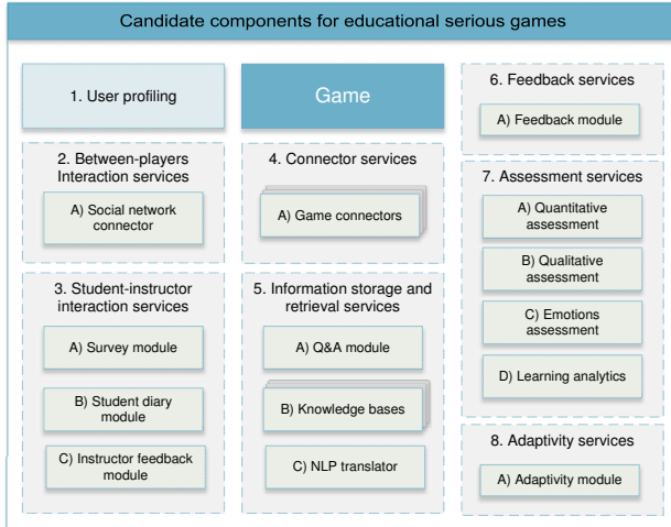
Fig. 2. The identified functional domains and their candidate components for implementation as services in a SOA framework for serious games
