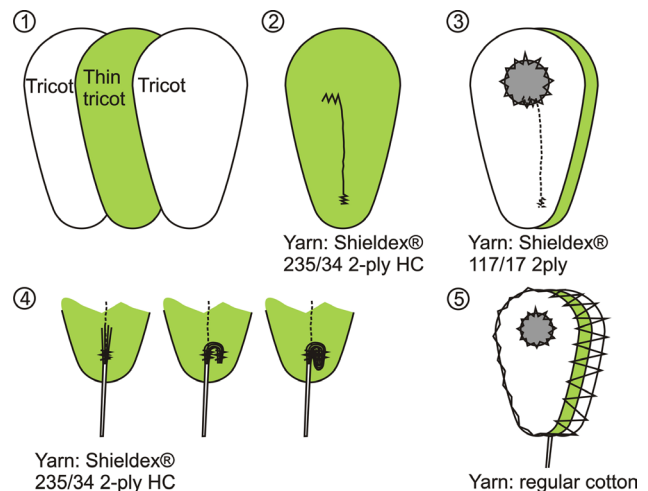
Fig. 3. Construction of textile electrodes
