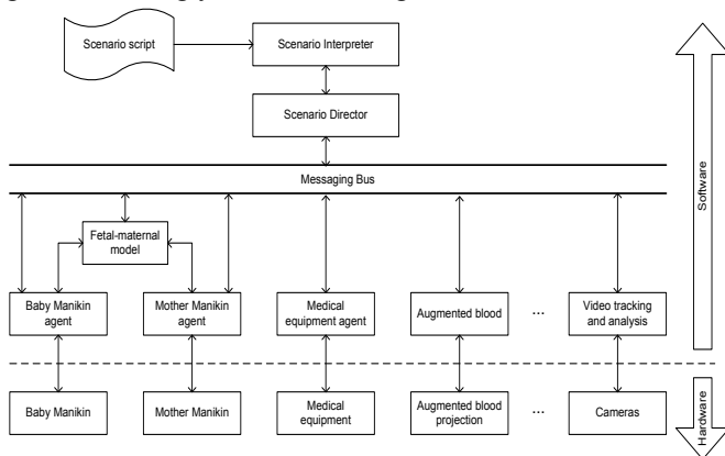
Fig. 12. MedSim system overview.
