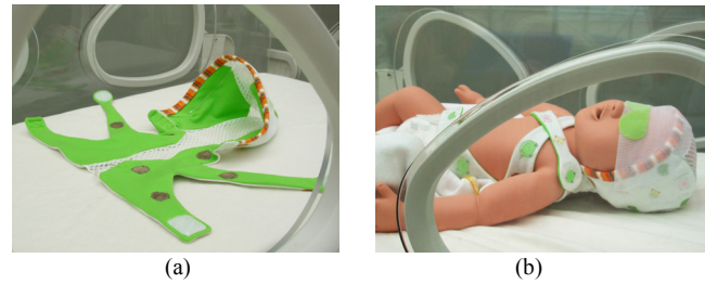
Fig. 1. (a) Prototype smart neonatal jacket, (b) a baby mannequin wearing the smart jacket inside the incubator.
